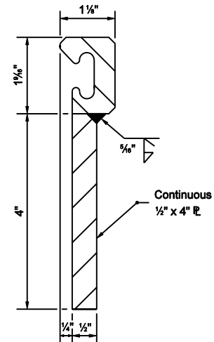
EXTRUSION & PLATE ASSEMBLY DETAIL
