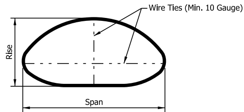
STEEL PIPE-ARCH SECTIONS END STABILIZATION OF 3" x 1" CORRUGATED ①
