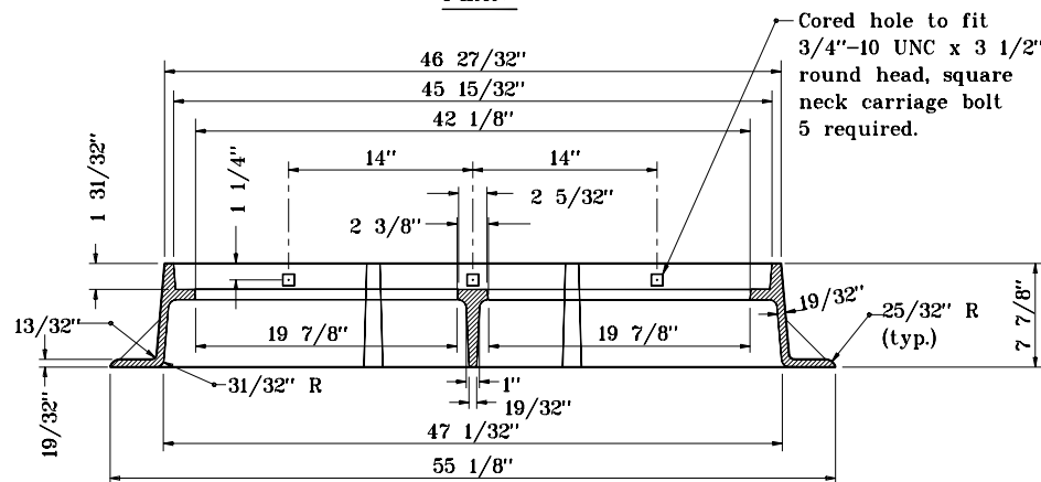
SECTION A-A FRAME CASTING TYPE 15
