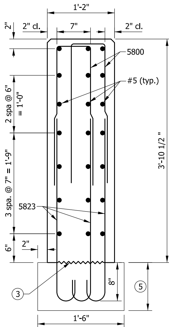
SECTION C-C
