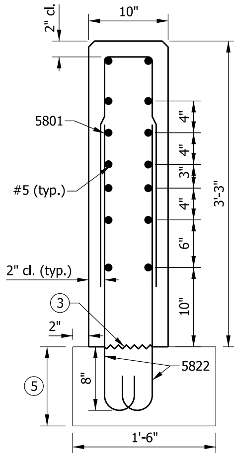
SECTION C-C
