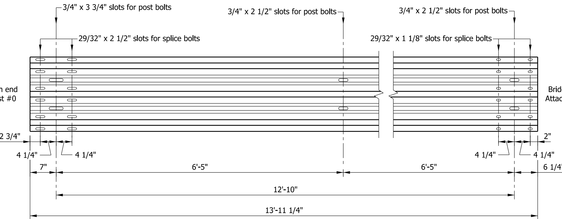
THRIE BEAM EXPANSION ELEMENT ELEVATION
