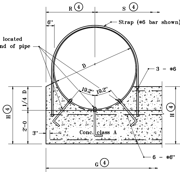
ANCHOR FOR CORRUGATED METAL PIPE PARTIAL ELEVATION
