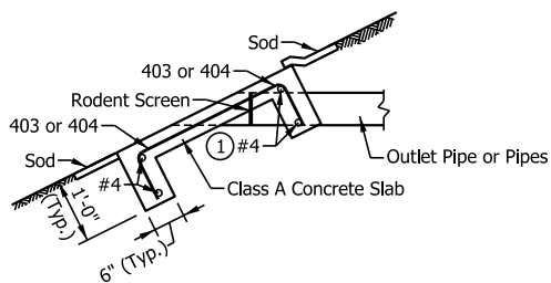
TYPICAL SECTION
